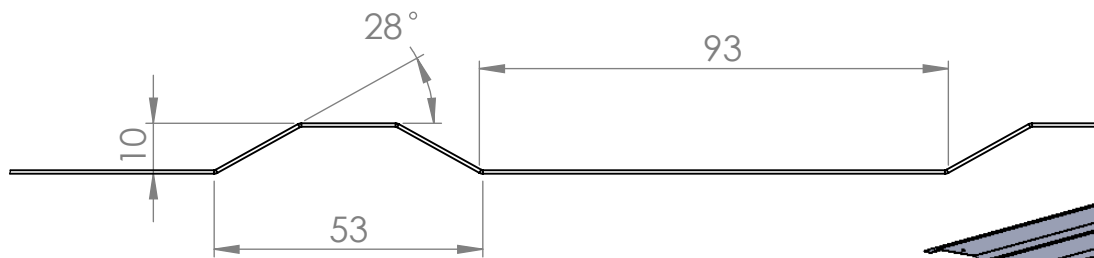
DETAIL A
